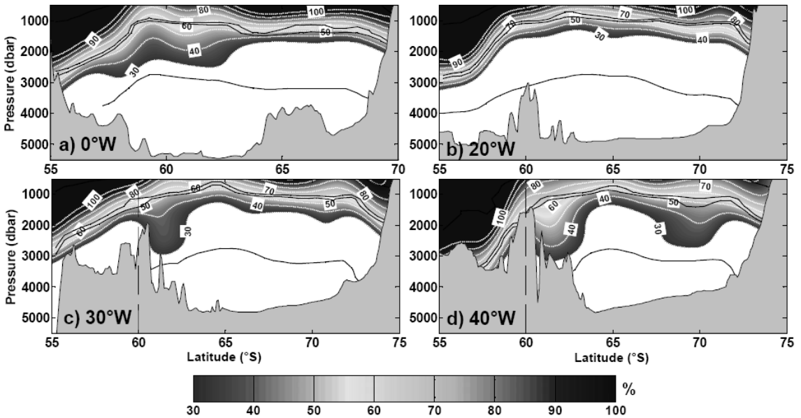
Fig. 4 – Warm Deep Water (WDW) contributions (%) at each meridional section analyzed as indicated by the annotations. Contour intervals are of 10% from 30% to 100%. The black lines indicate the neutral density ( \gamma^n ) isopycnals of 28.10, 28.26, 28.27, and 28.4 \text{kg}\cdot\text{m}^{-3} for 0°, 20°W, 30°W, and 40°W, respectively. The dashed line shows the limit between the Scotia and Weddell Seas at 30°W and 40°W.
