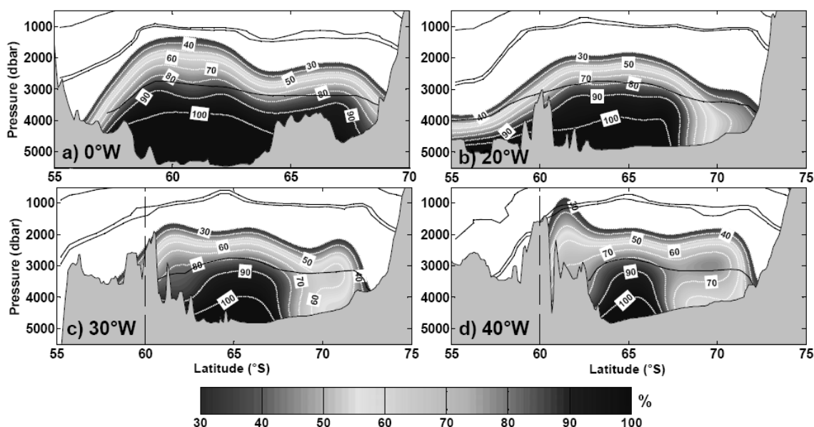
Fig. 6 – Same as Figure 4, but for Weddell Sea Bottom Water (WSBW).
