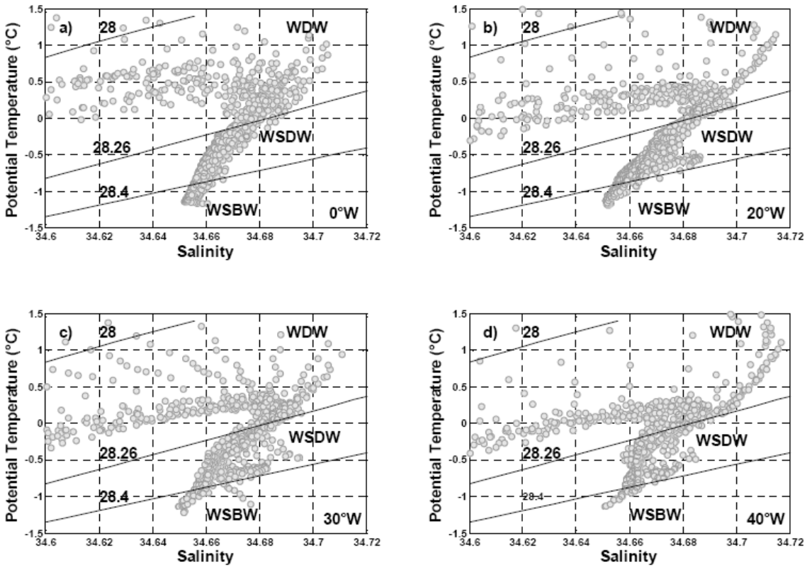
Fig. 3 – SODA potential temperature-salinity diagram for the meridional transects analyzed as indicated at the bottom of each box. Neutral density values of 28, 28.26, and 28.4 kg·m -3 were selected as AASW/WDW, WDW/WSDW and WSDW/WSBW interfaces, following Franco et al. (2007).
