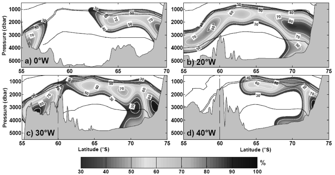
Fig. 5 – Same as Figure 4, but for Weddell Sea Deep Water (WSDW).
