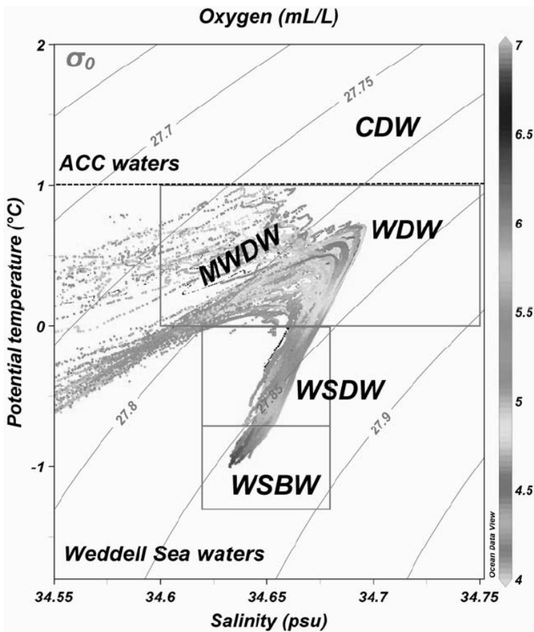
Fig. 2 – World Ocean Database 2005 potential temperature-salinity-dissolved oxygen diagram for Weddell Sea deep water masses below 200 m of depth. The straight lines show potential density ( \sigma_\theta ) surfaces and the dashed line marks the limit between Weddell Sea and Antarctic Circumpolar Current (ACC) deep waters. Water mass limits (rectangles) of Weddell Sea and ACC regions are based on Robertson et al. (2002) property definitions.
