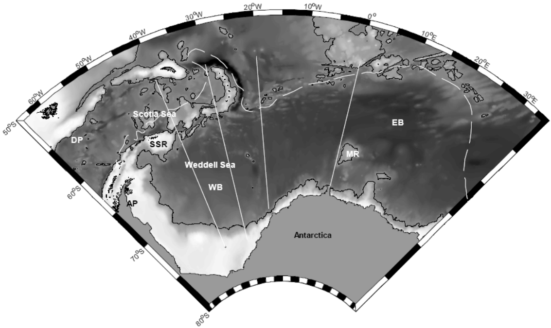
Fig. 1 – Study area in the Weddell Sea (WS) and Weddell-Scotia Confluence region. The thicker white lines show the repeat hydrographic sections selected to run OMP. The dashed white line shows de Southern Boundary of the ACC (as in Orsi et al. 1995). The black line shows the 3000m isobaths. Antarctic Peninsula (AP), Drake Passage (DP), Enderby Basin (EB), Maud Rise (MR), South Scotia Ridge (SSR), Weddell Basin (WB).
